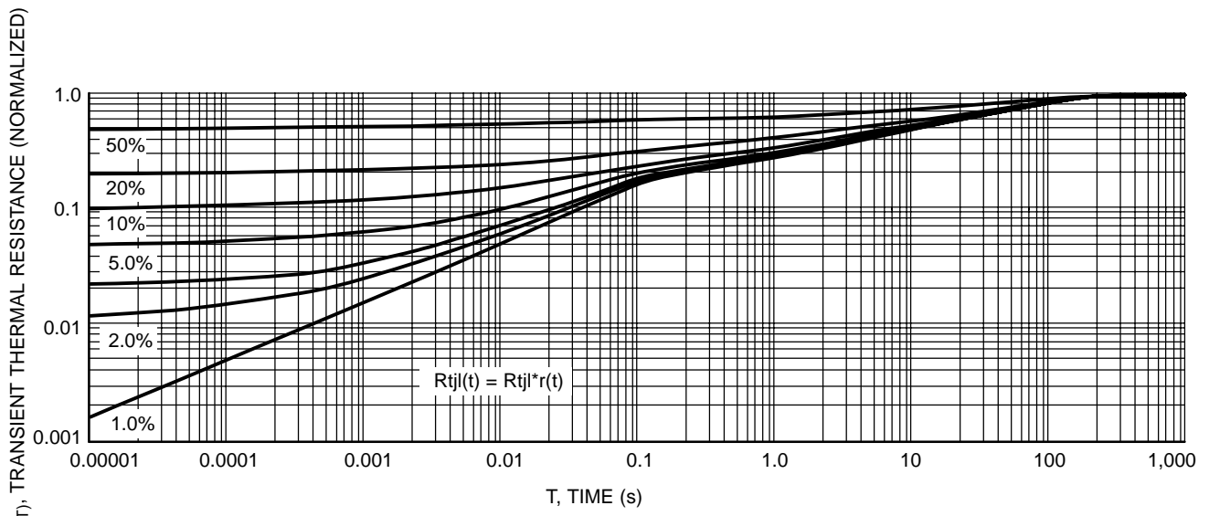
Figure 10. Thermal Response Junction to Ambient
